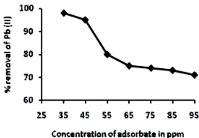
Fig. 7. Effect of initial metal ion concentration on removal of lead (II) ions; temperature: 27 °C; agitation speed: 200 rpm; contact time: 120 min.; dose of adsorbent: 1g/L; pH: 6; initial sorbate concentration: 35-95 mg/L.
