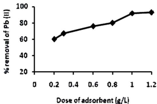
Fig. 5. Effect of dose of adsorbent GDCC on removal of lead (II) ions. Initial Pb^{2+} concentration: 35 mg/L; pH: 6; temperature: 27 °C; agitation speed: 200 rpm.; contact time: 120 min.; dose of adsorbent: 0.2 g to 1.2 g.
