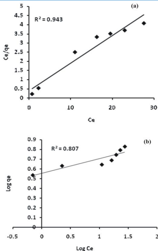
Fig. 8. (a) Langmuir adsorption isotherm, (b) Freundlich adsorption isotherm.
