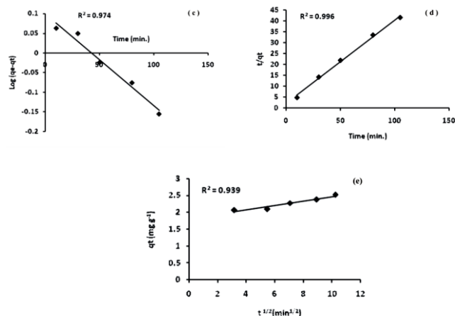
Fig. 8. (c) Pseudo first order kinetic plot, (d) Pseudo second order kinetic plot and (e) Intraparticle diffusion model.
