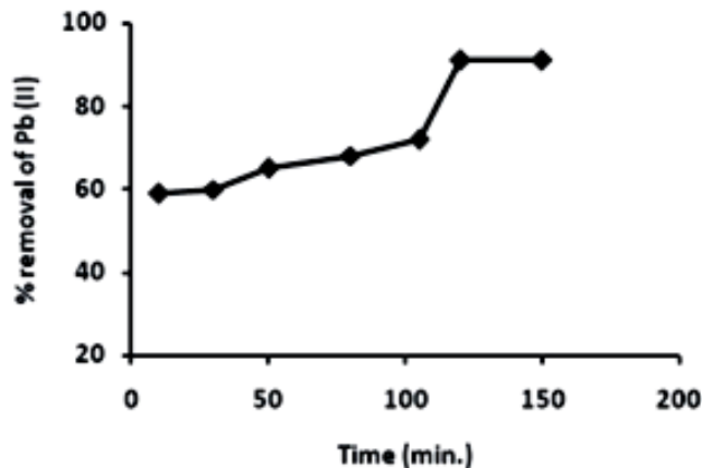
Fig. 4. Effect of contact time of GDCC on removal of lead (II) ions. Initial Pb^{2+} concentration: 35 mg/L; pH: 6; temperature: 27 °C; agitation speed: 200 rpm.; dose of adsorbent: 1 g/L; contact time: 10 to 150 min.
