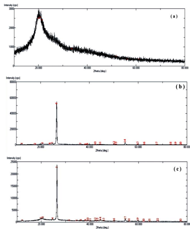
Fig. 2. Powder XRD pattern of (a) chitosan (b) graphite (c) graphite doped chitosan composite.
