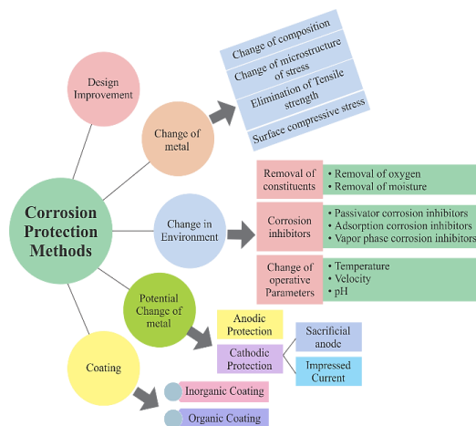
Fig. 1. Methods for corrosion inhibition.
